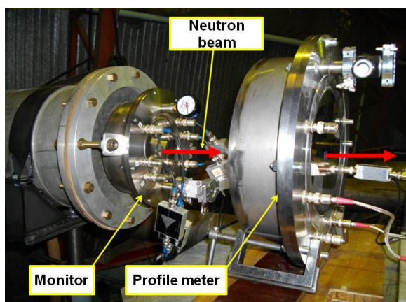
Figure 4: FIC (neutron monitor) and MWPC (profile meter).
